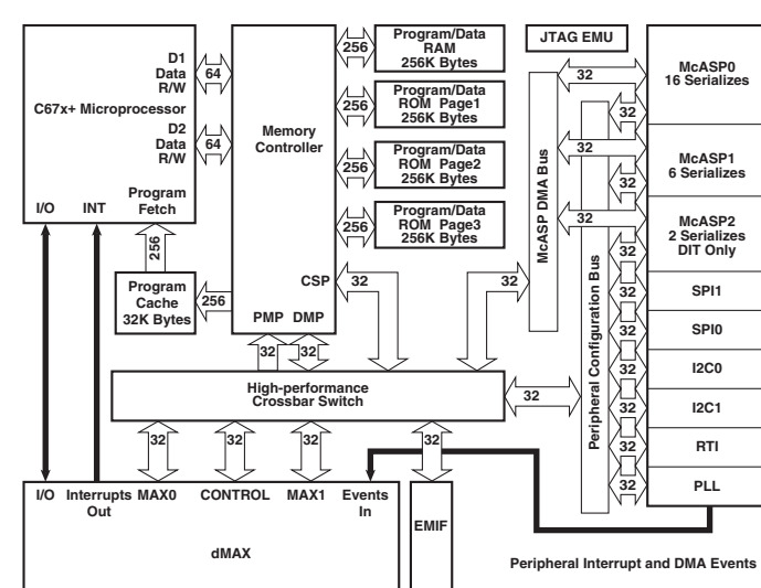
IC241: D70YE101BRFP266 Floating-point digital signal processors
