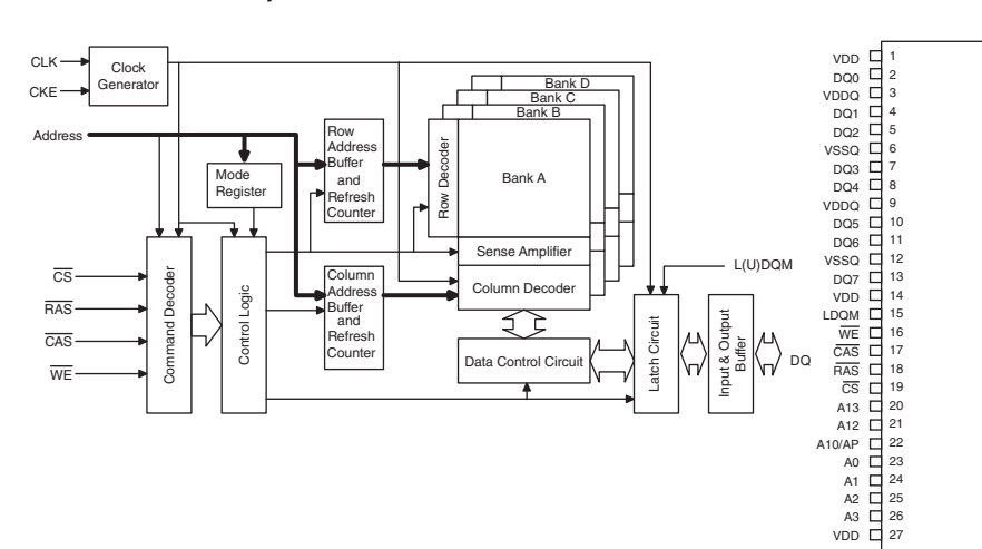
IC242: M12L64164A-5TG 1M x 16-bit x 4 banks synchronous DRAM
