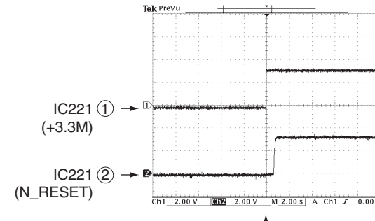
POINT ③ ①/ IC221 (97 pin, +3.3M), ②/ IC221 (10 pin, N_RESET)
