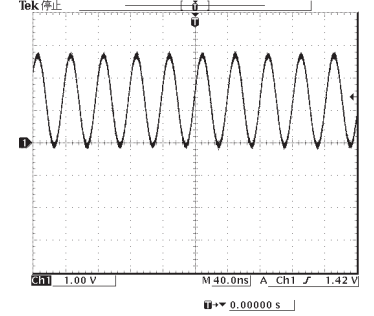
POINT ④ XL261 (Pin 29 of IC261)
