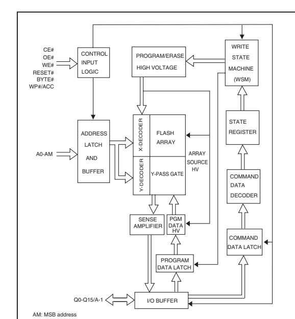
IC243: MX29LV160DBT1-70G 16M-bit 3V supply flash memory
