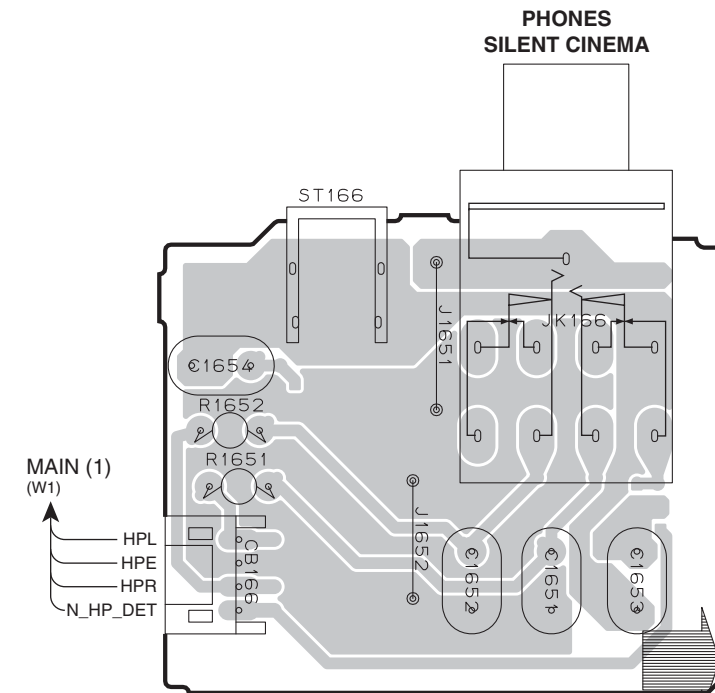
OPERATION (5) P.C.B. (Side A)
